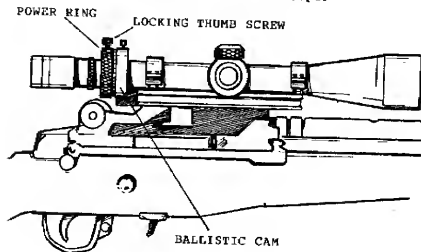
Figure 2-15. ART II scope.
